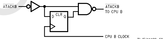
FIGURE 33c. Modifying Wait Logic for Port B
