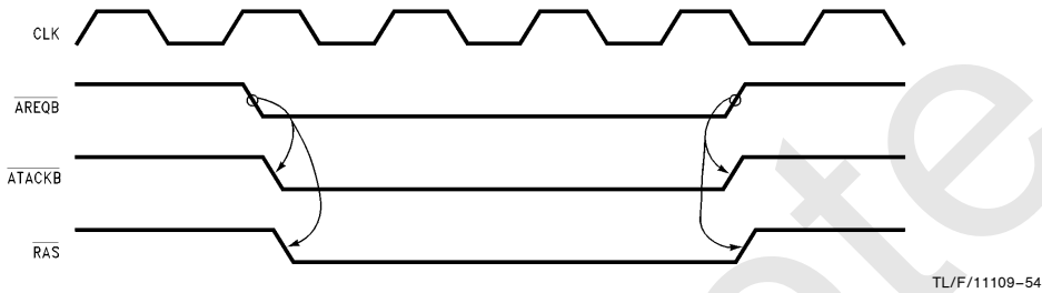
FIGURE 33a. Non-Delayed Port B Access
