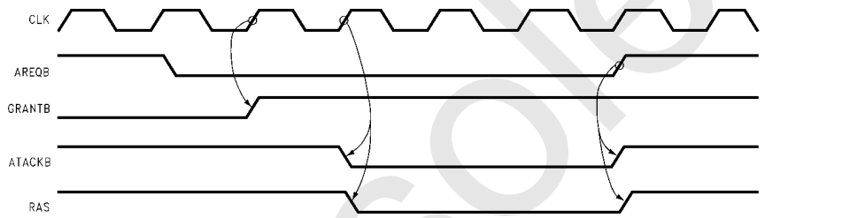
FIGURE 33b. Delayed Port B Access
