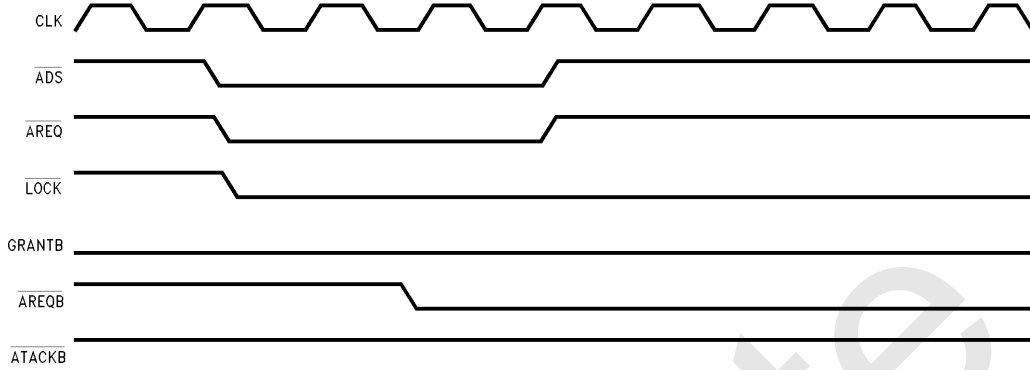
FIGURE 35. \overline{\text{LOCK}} Function
