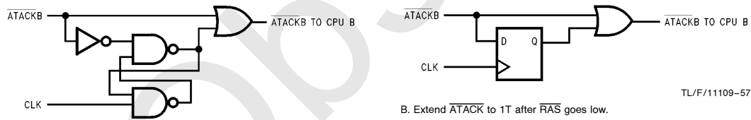
FIGURE 33b. Delayed Port B Access
