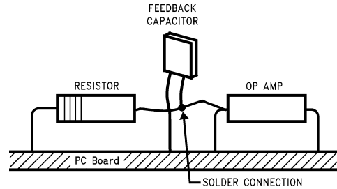
Figure 29. Air Wiring
