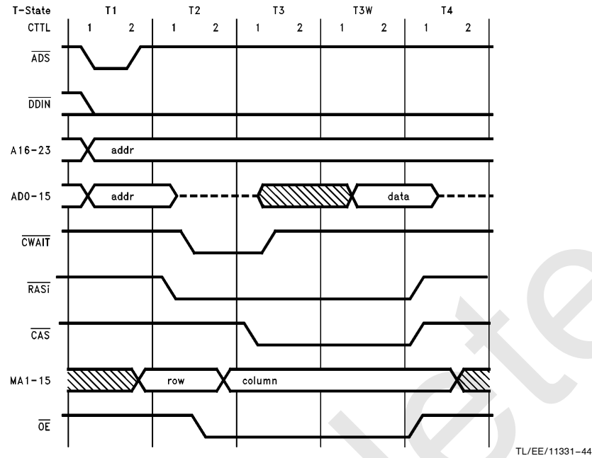
FIGURE 3-12. Zone 2 (DRAM) Read Transaction, One Wait State
