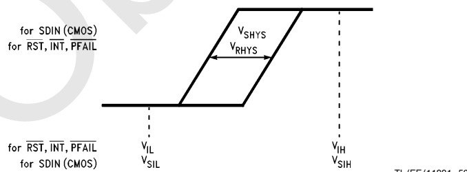
FIGURE 4-7. Input Hysteresis
