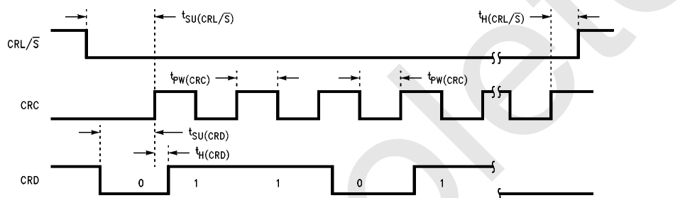
FIGURE 4. MICROWIRE™ Compatible Control Register Serial Load Timing Diagram
