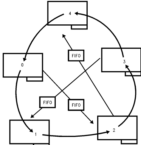
FIGURE 2.2. Logical Data flow (QuickRing Virtual FIFOs)
