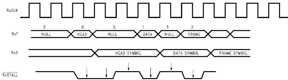
FIGURE 3.11. Null Type is Inserted when \overline{\text{RxSTALL}} is Asserted during the same Clock Cycle as a Null Symbol (i.e., in above Figure Null is Inserted after Head Symbol, see also Table 3.0 State #9)
