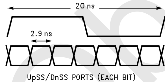
FIGURE 2.4. A Sub-Symbol is Multiplexed Every 2.9 ns
