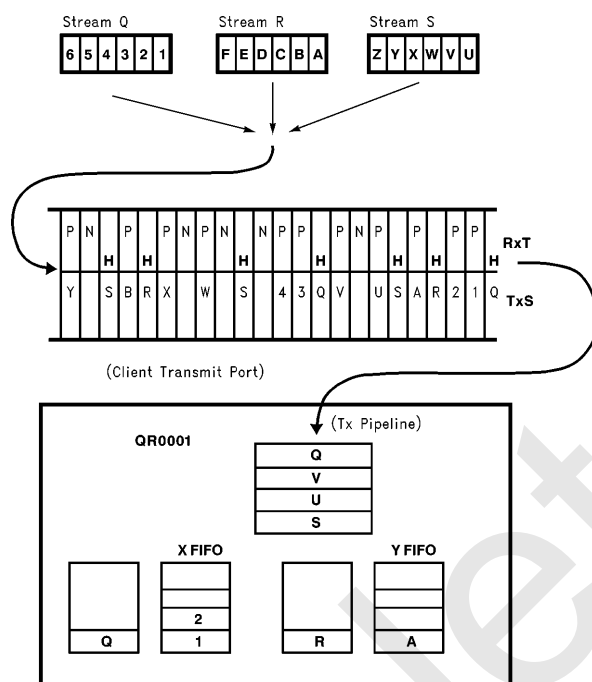
FIGURE 3.3. Logically Distinct Streams of Data can be Multiplexed Into the Tx Port
