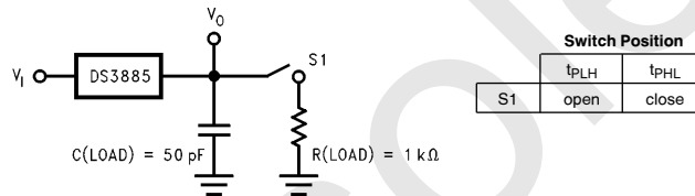
FIGURE 4. Receiver Propagation Delay Set-Up
