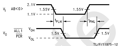
FIGURE 8. AB0 to ALL1, AB0 to \overline{PER}
