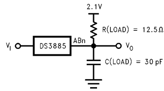
FIGURE 1. Driver Propagation Delay Set-up
