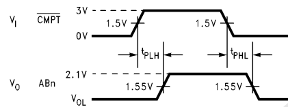
FIGURE 3. Driver: CMPT to AB7
