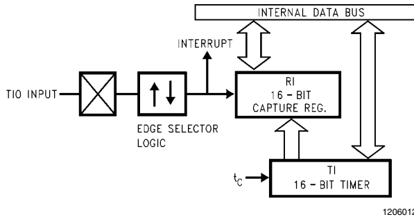
FIGURE 9. Timer in Input Capture Mode
