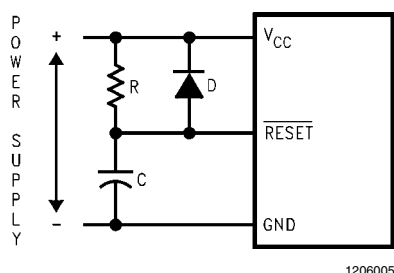
FIGURE 3. Recommended Reset Circuit
