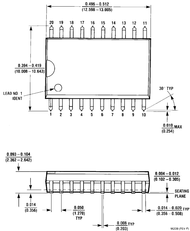
20-Lead Molded Small Outline Package (M) Order Number COP912C-XXX/WM, COP912CH-XXX/WM NS Package Number M20B
