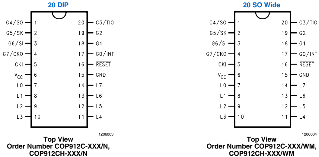
FIGURE 2. COP912C/COP912CH Pinout
