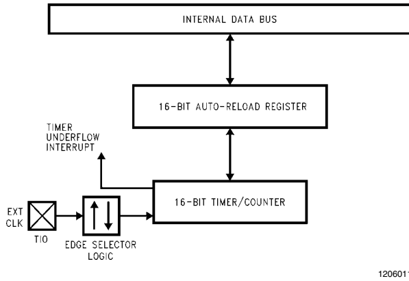
FIGURE 8. Timer in External Event Mode
