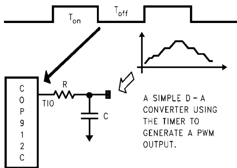
FIGURE 10. Timer Based PWM Application
