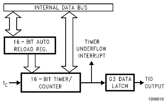
FIGURE 7. Timer in PWM Mode
