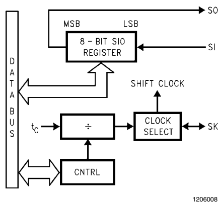
FIGURE 6. MICROWIRE/PLUS Block Diagram
