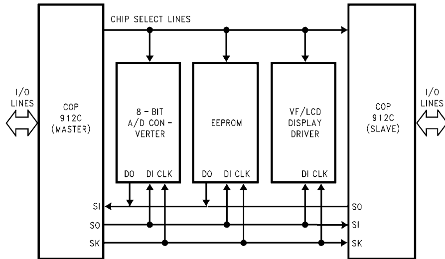
FIGURE 5. MICROWIRE/PLUS Application
