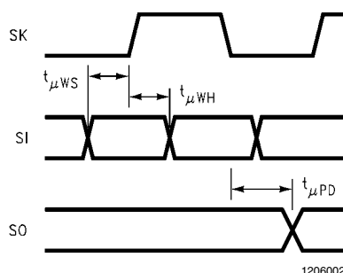
FIGURE 1. MICROWIRE/PLUS Timing
