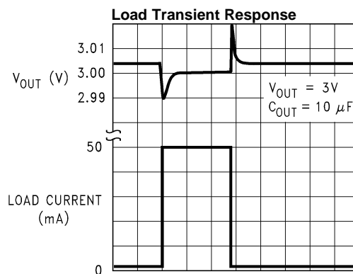
10 \mu\text{s}/\text{div} → Figure 19.
