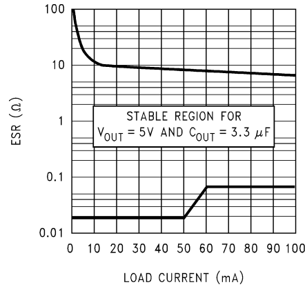
Figure 34. 5V/3.3 μF ESR Curves
