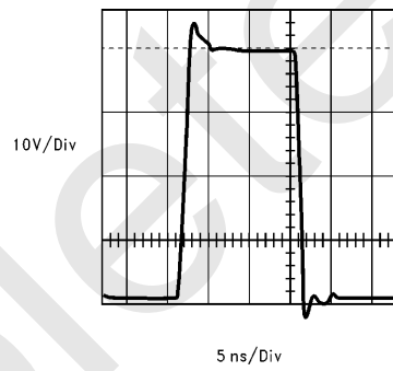
FIGURE 6. Pulse Response
