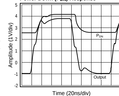
Power Down ( P_{DN} ) Response
