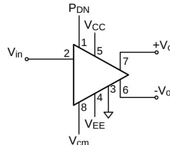
Figure 4: CLC503 Functional Pin Descriptions
