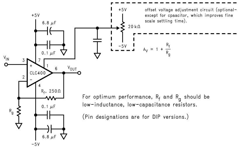
Figure 17. Recommended Non-Inverting Gain Circuit
