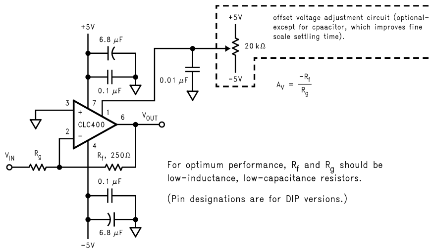
Figure 18. Recommended Inverting Gain Circuit
