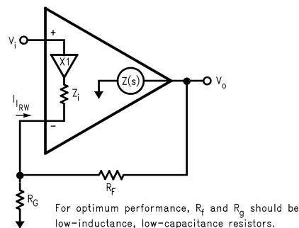
Figure 19. Current Feedback Topology
