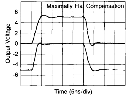
Settling Time into a 50\text{pF} Load
