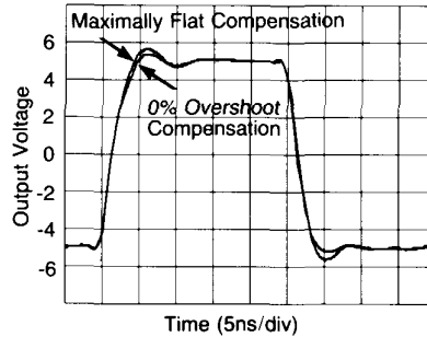
Settling Time into 500\Omega Load
