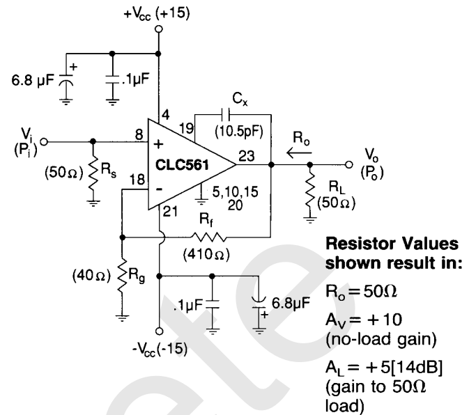
Figure 1: Test Circuit
