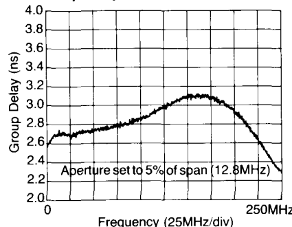
Group Delay
