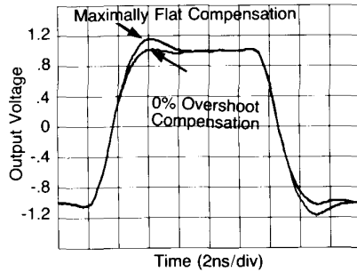
Settling Time into 50\Omega Load
