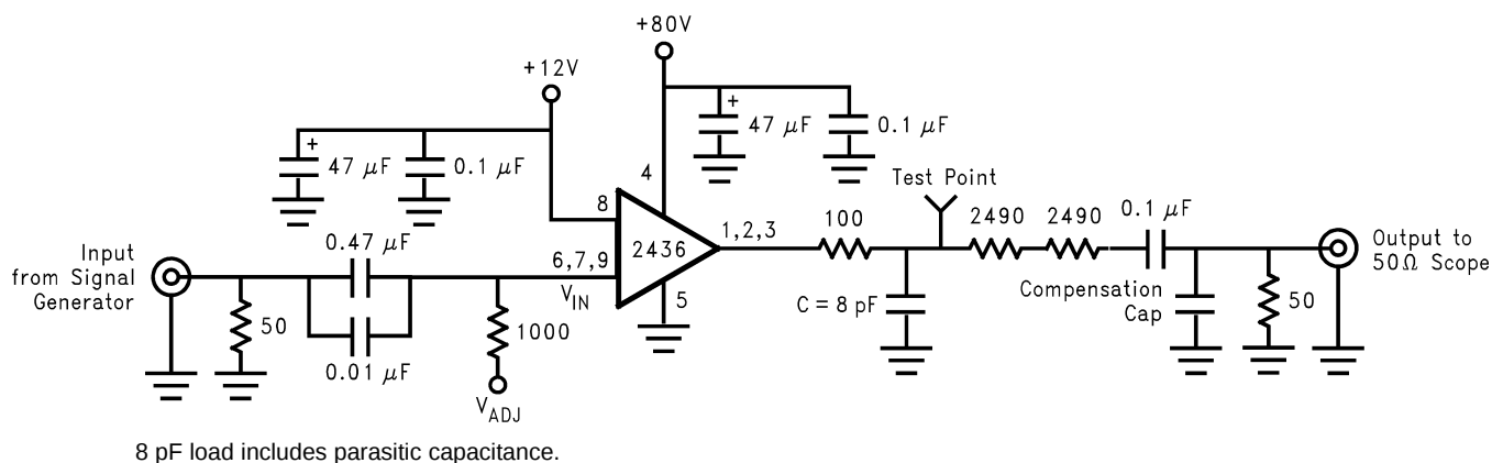
Figure 2. Test Circuit (One Channel)
