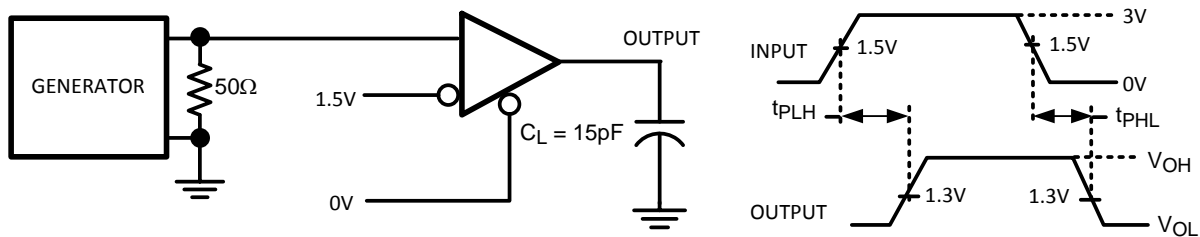
Figure 8. Test Circuit for Receiver T_{PLH} and T_{PHL}
