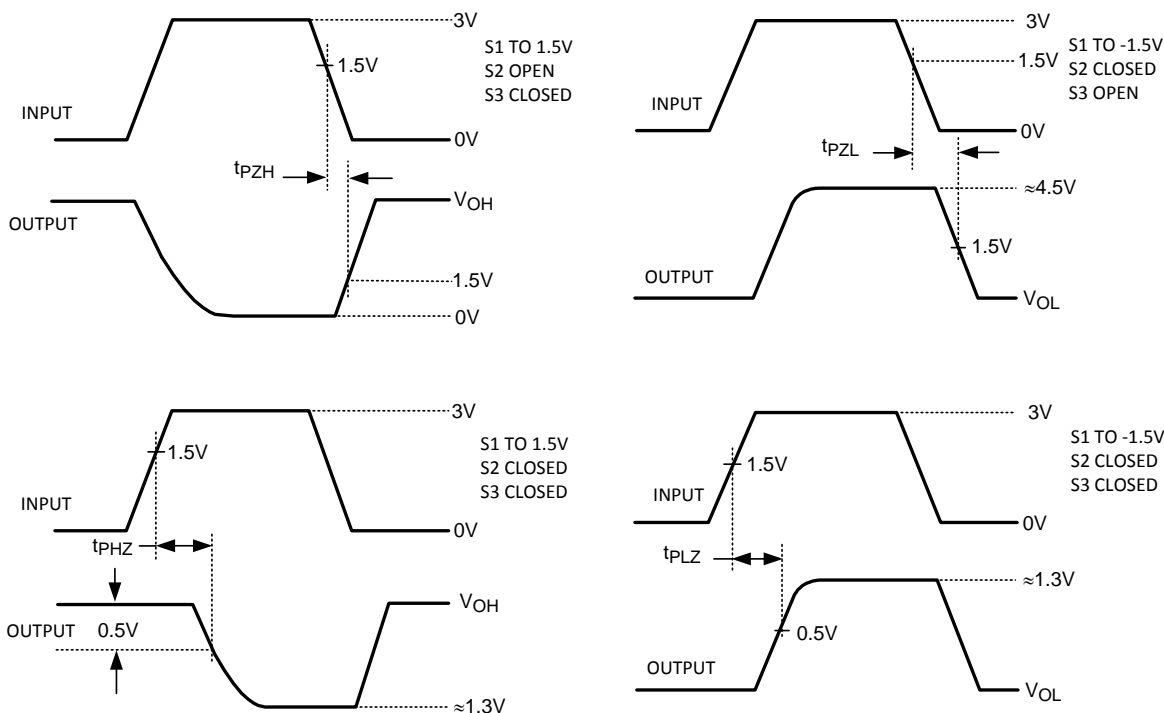
VOLTAGE WAVEFORMS
