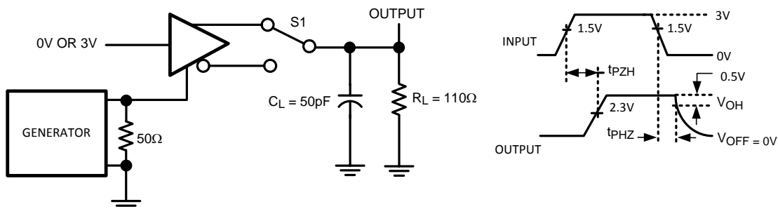
Figure 5. Test Circuit for Driver T_{PZH} and T_{PHZ}
