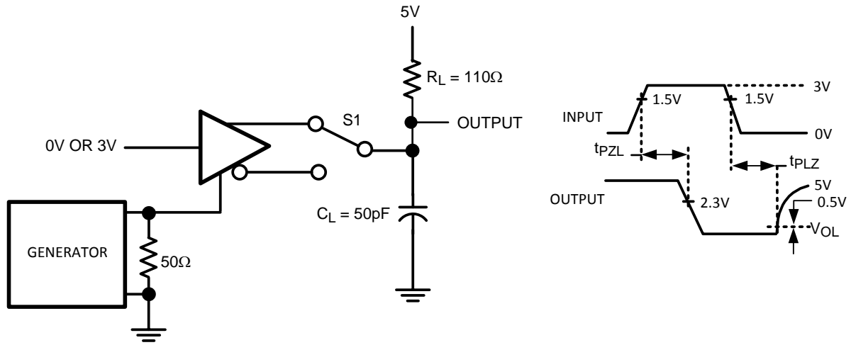
Figure 6. Test Circuit for Driver T_{PZL} and T_{PLZ}
