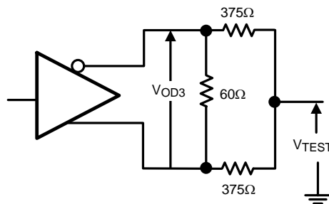
Figure 3. Test Circuit for V_{OD2}
