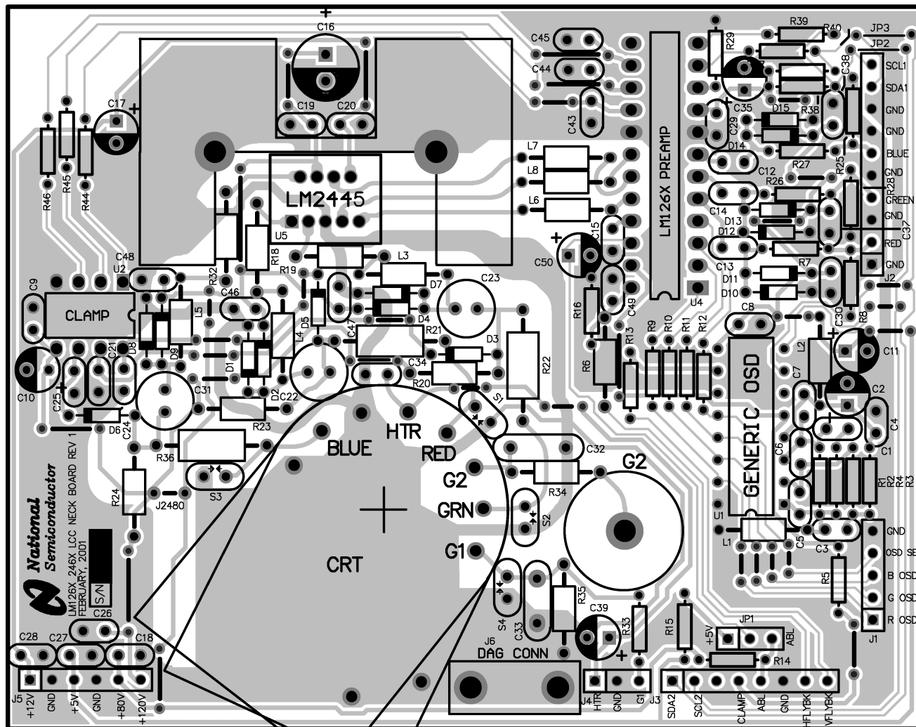
Figure 14. LM126X/LM246X Demo Board Layout
