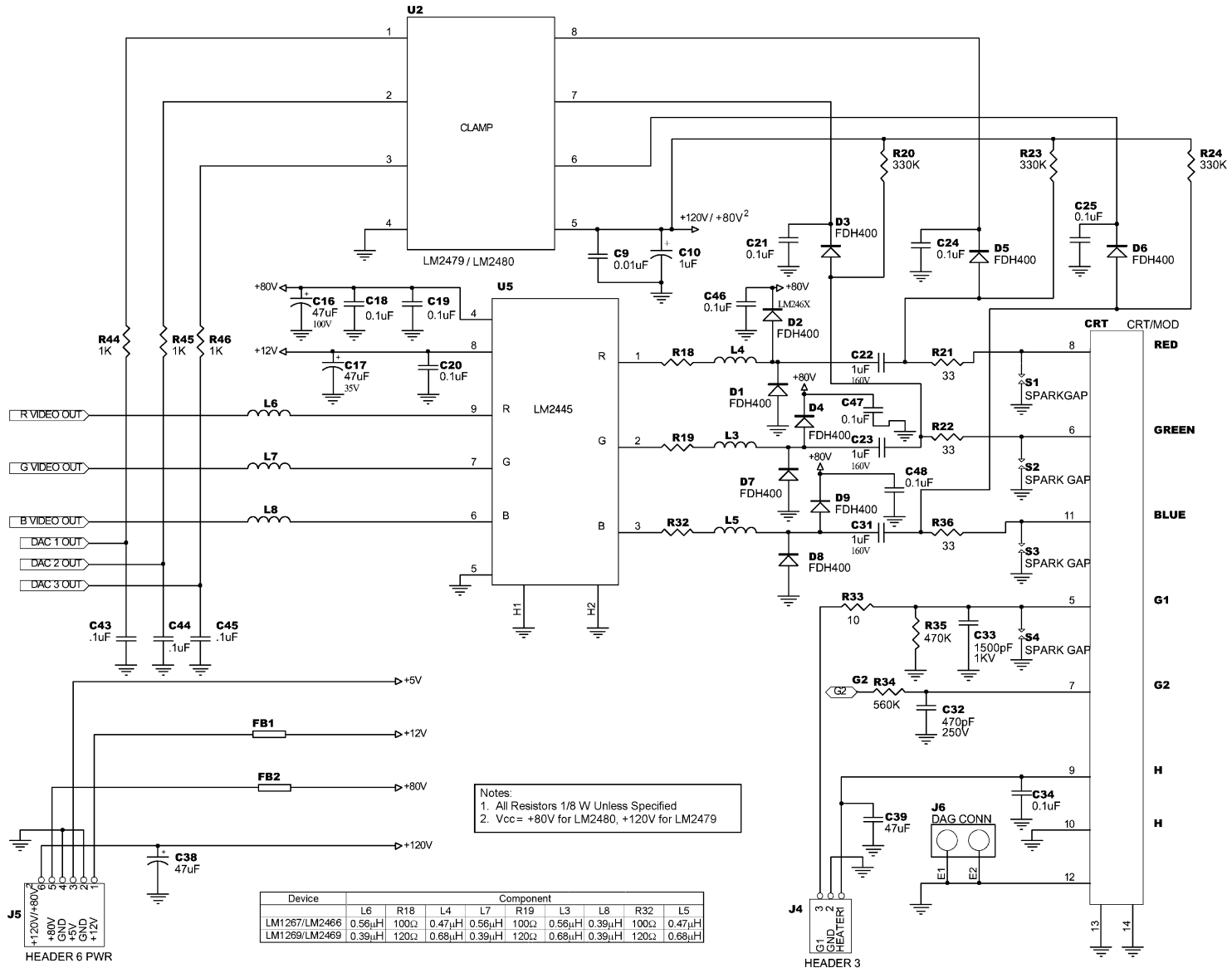
Figure 13. LM126X/LM246X Demonstration Board Schematic (continued)
