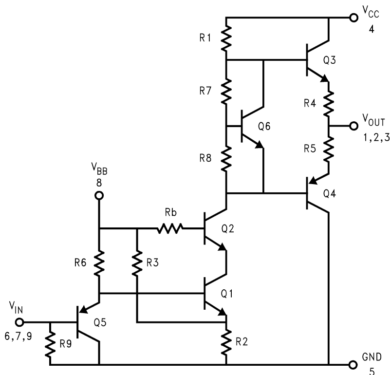
Figure 1. Simplified Schematic Diagram (One Channel)
