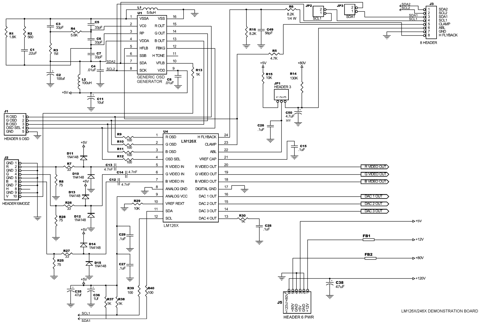
Figure 12. LM126X/LM246X Demonstration Board Schematic
