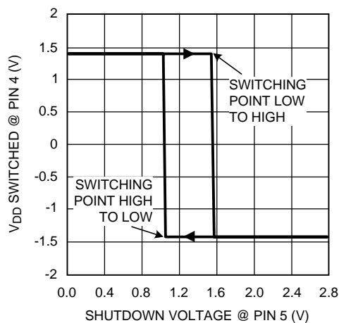
Figure 33. Hysteresis
