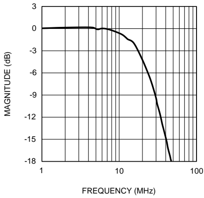
Figure 6. Bandwidth
