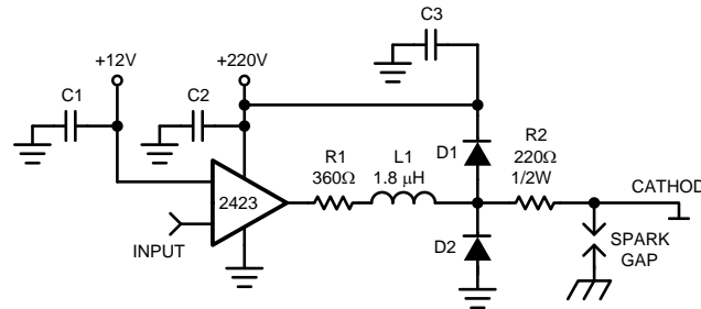
Figure 13. One Channel of the LM2423 with the Recommended Application Circuit
