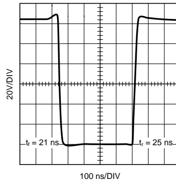
Figure 12. LM2423 Cathode Response
