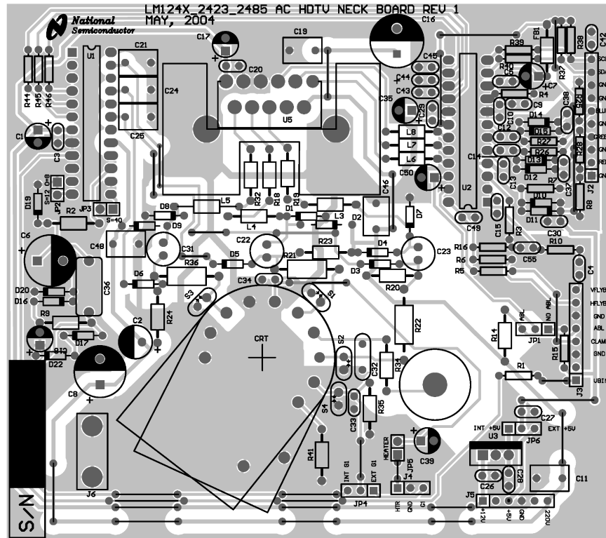
Figure 15. LM2423/LM1246/LM2485 DTV Demonstration Board Layout
