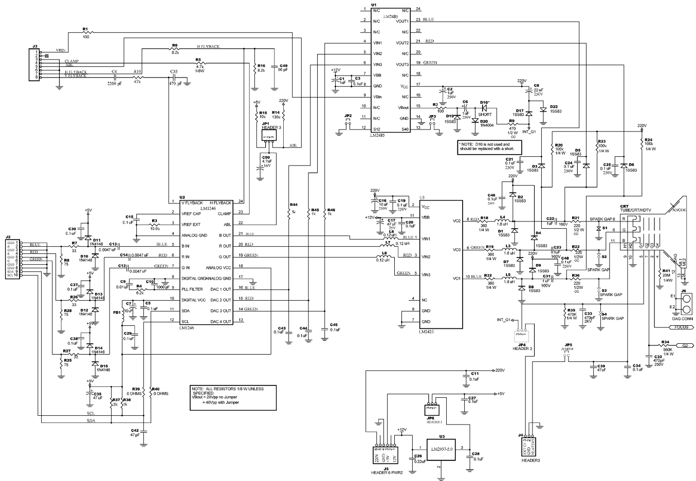
Figure 14. LM2423/LM1246/LM2485 DTV Applications Circuit
