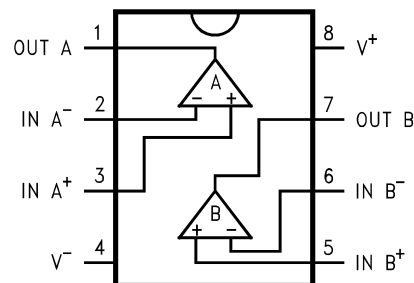
Figure 3. 8-Pin VSSOP Top View
