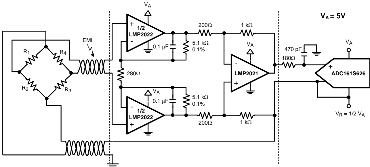
Figure 50. LMP2021/LMP2022 used with ADC161S626
