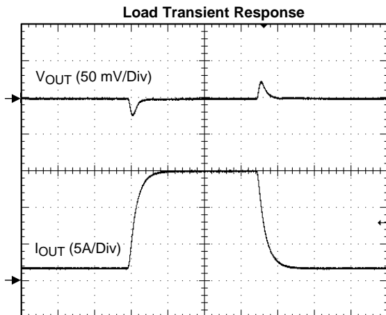
Figure 19. 100 μs/DIV
