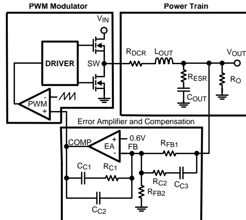
Figure 33. Loop Diagram
