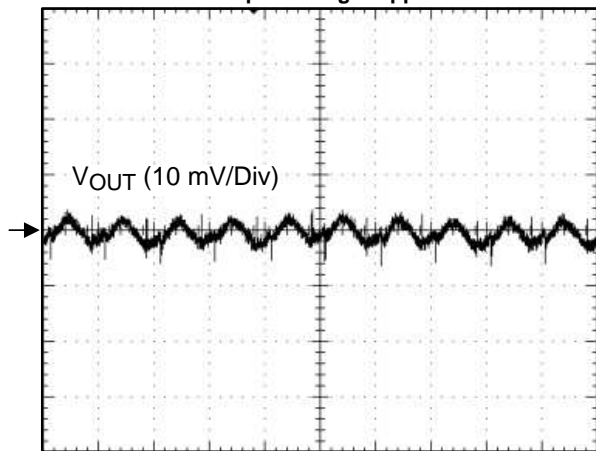
Figure 20. 2 \mu s /DIV
