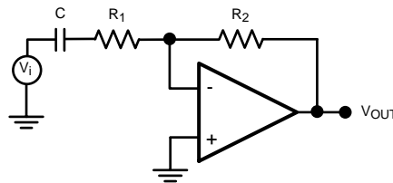
Figure 46. Highpass Filter
