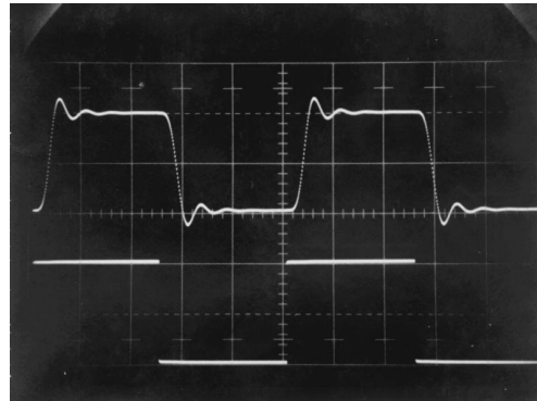
FIGURE 18. MF6-50 Step Input Response, Vertical = 2V/div, Horizontal = 1 ms/div, f_{CLK} = 100 kHz
