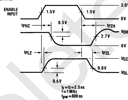
FIGURE 4. TRI-STATE Control Levels
