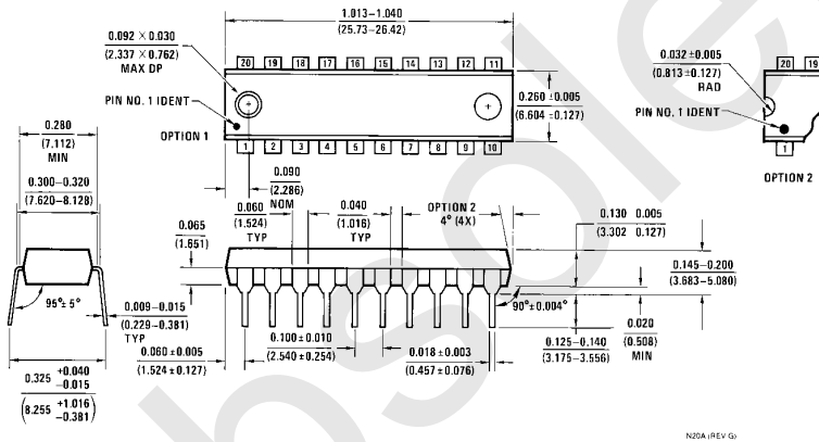
20-Lead Dual-In-Line Package (N) Order Number DP84240N/DP84244N NS Package Number N20A
