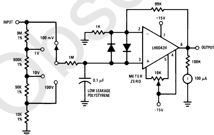
Sensitive Low Cost "VTVM"
