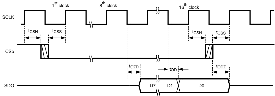
Figure 54. Read Timing
