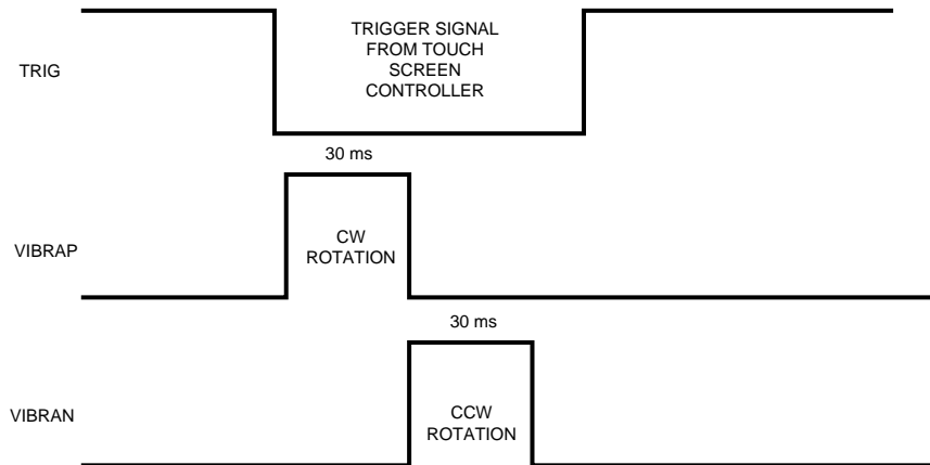
Figure 30. Control Waveform
