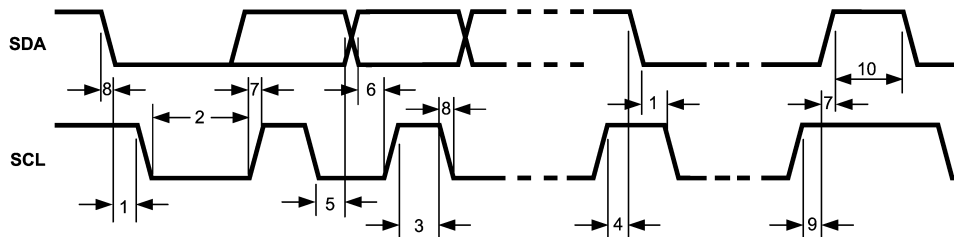
Figure 2. Timing Parameters
