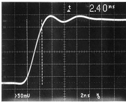
FIGURE 17. LM1208 Rise Time
