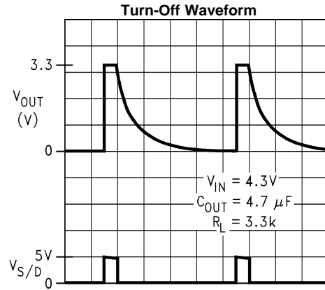
20 \text{ms}/\text{Div} Figure 17.
