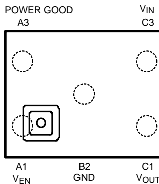
Figure 2. Top View 5 Bump DSBGA Package (YZR) See Package Number YZR0005
