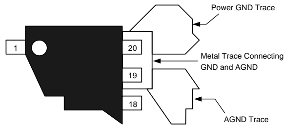
Figure 43. Single Layer Layout
