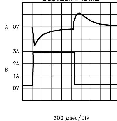
Figure 18. Horizontal Time Base: 200 \mu s/div
