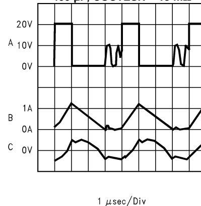
Figure 16. Horizontal Time Base: 1 \mu s/div
