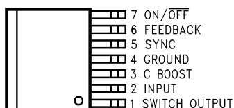
Figure 1. DDPACK Package- Top View See Package Number KTW
