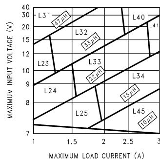
Figure 22. LM2670-5.0EP
