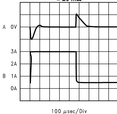
Figure 17. Horizontal Time Base: 100 \mu s/div
