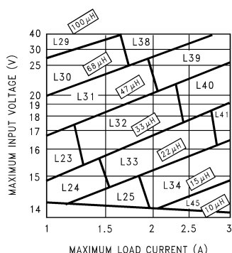
Figure 23. LM2670-12EP
