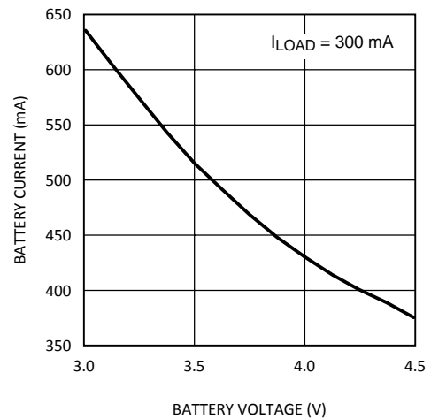
Figure 12. Battery Current vs Voltage
