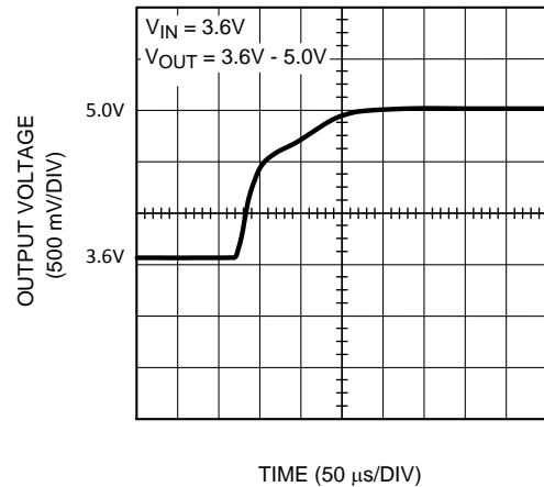
Figure 14. Boost Startup with No Load
