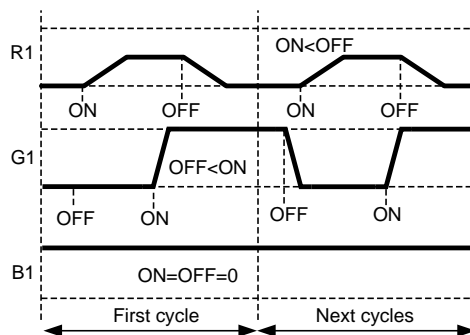
Figure 19. Example Blinking Waveforms
