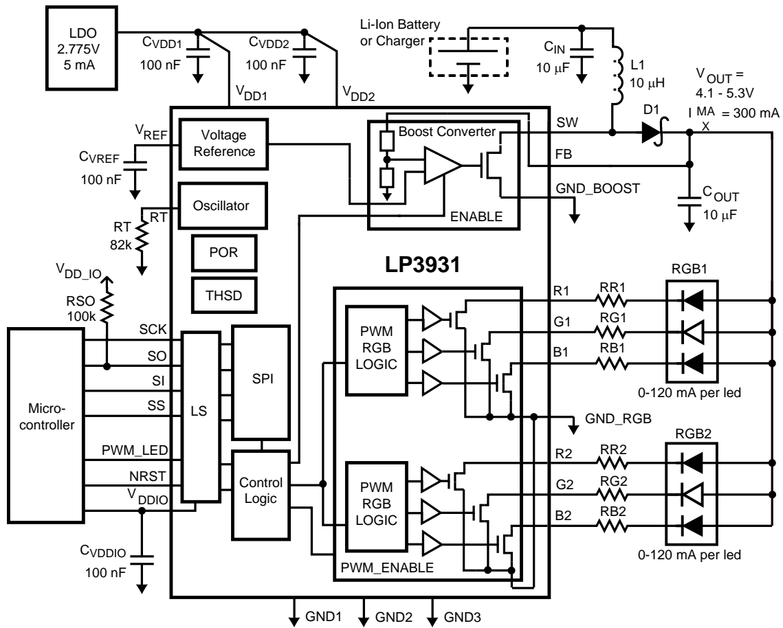
Figure 3. LP3931 Block Diagram
