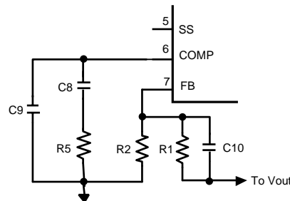
Figure 24. Compensation Network
