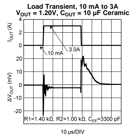
10 \mu\text{s}/\text{DIV} Figure 12.
