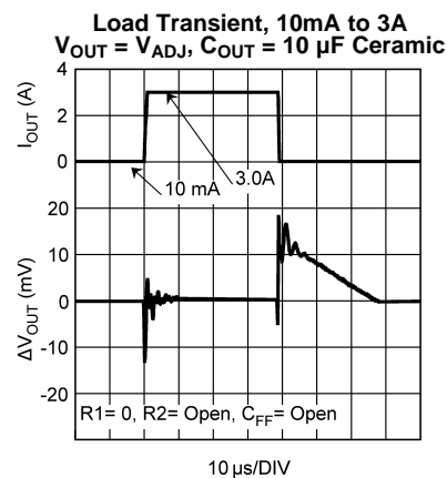
10 \mu\text{s}/\text{DIV} Figure 11.
