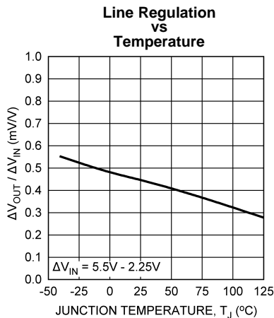
\Delta V_{IN} = 5.5\text{V} - 2.25\text{V} Figure 9.
