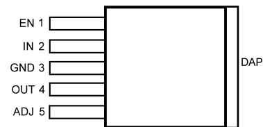
Figure 2. 5-Pin DDPAK/TO-263, Top View (LP38502TS-ADJ) See KTT0005B Package
