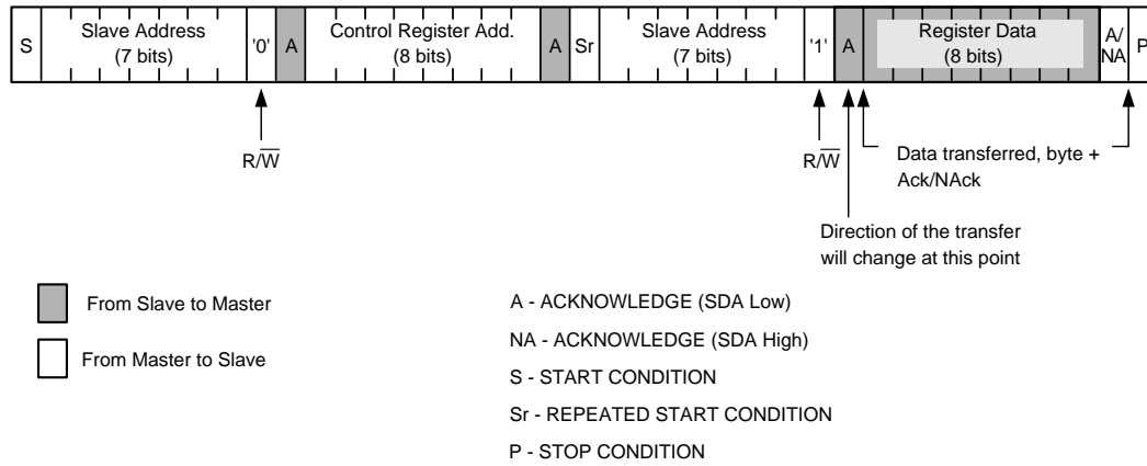
Figure 8. Register Read Format
