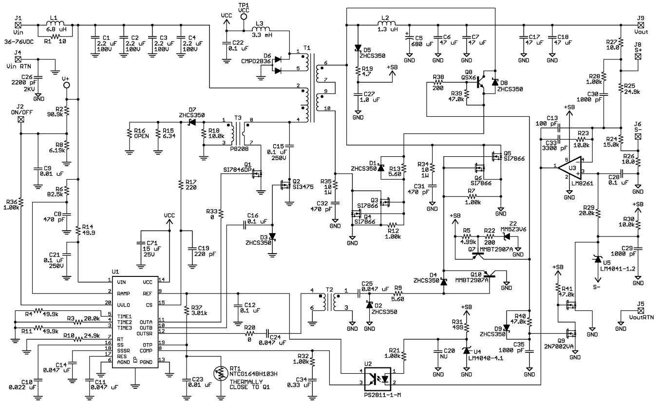
Figure 35. Application Circuit
