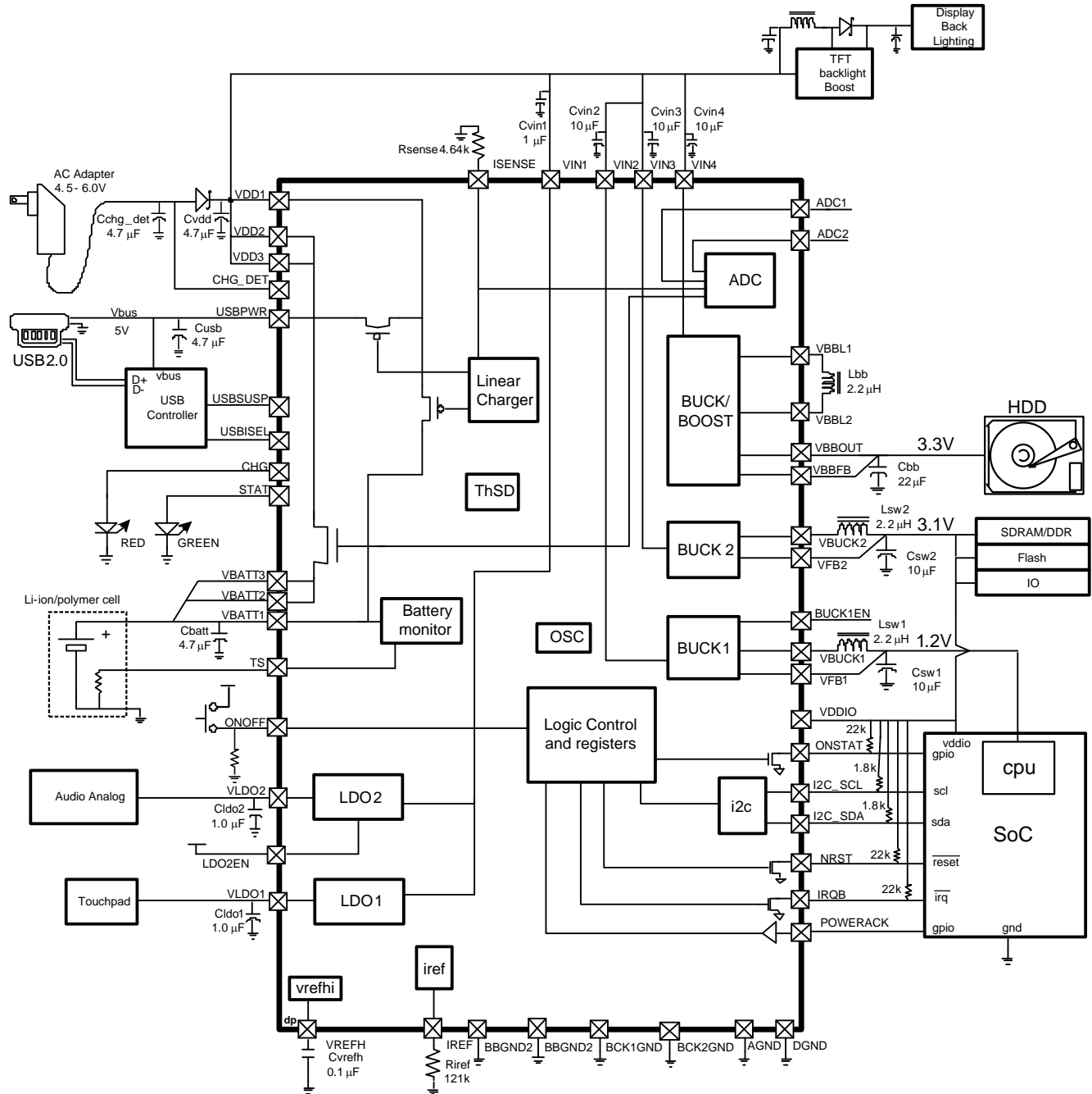
Figure 1. Application Diagram
