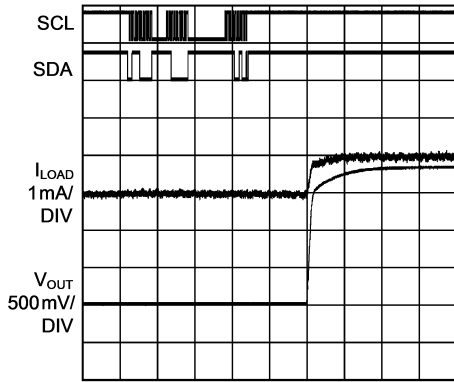
Regulator 2,3,4 Short Circuit Current V_{OUT} setting = 1.80V
