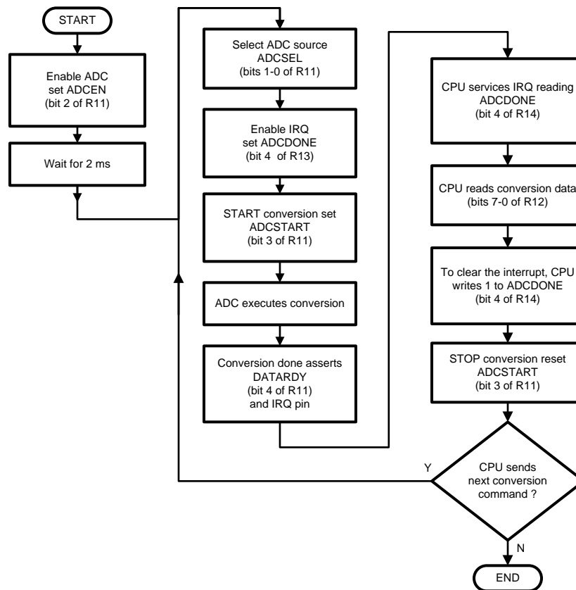
Figure 36. ADC Operation
