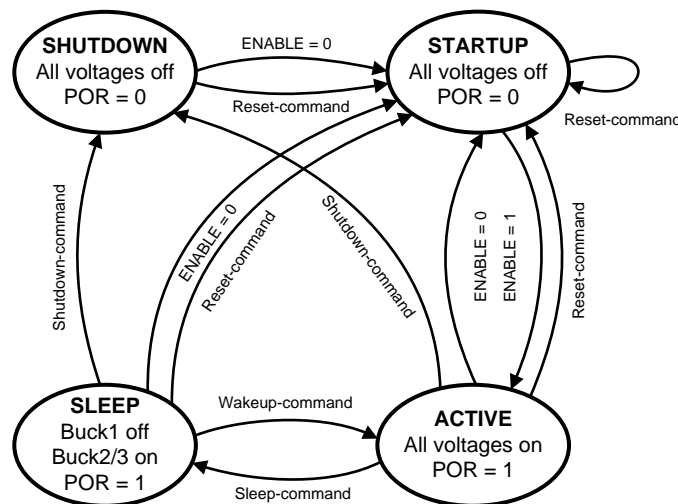
Figure 33. LM10503 State Diagram
