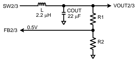
Figure 29. Bucks2/3 V_{OUT} Adjust
