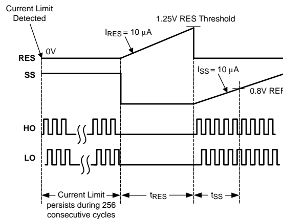
Figure 27. Hiccup Mode Current Limit Timing Diagram
