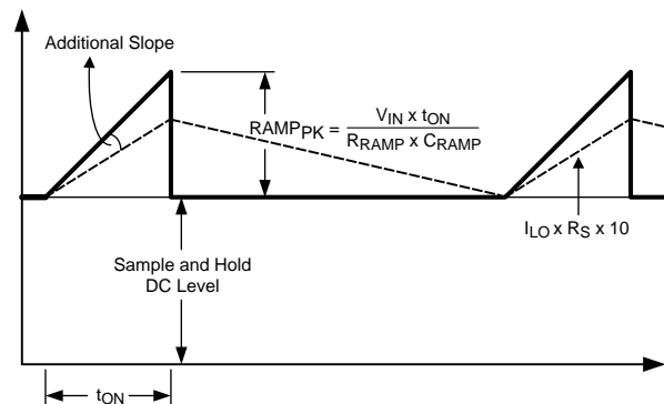
Figure 23. Composition of Emulated Current Sense Signal
