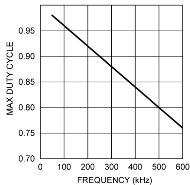
Figure 31. Maximum Duty Cycle vs Switching Frequency
