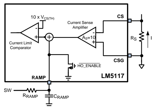
Figure 24. RAMP Generator and Current Limit Circuit
