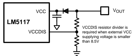
Figure 19. External VCC Supply for 6V < V_{OUT} < 14.5V
