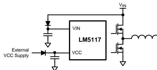
Figure 18. VIN Configuration for V_{VIN} < V_{VCC}
