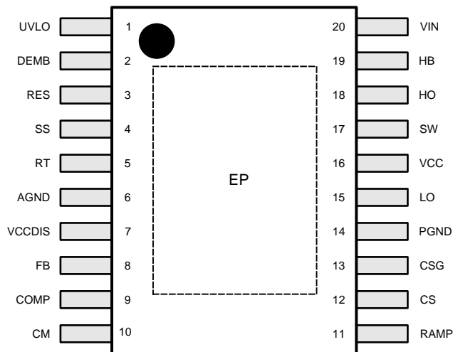
Figure 1. 20-Lead HTSSOP Package (Top View)
