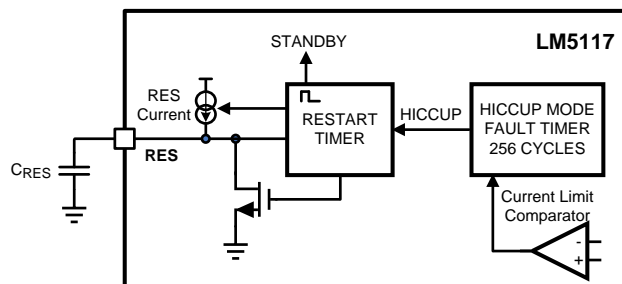
Figure 28. Hiccup Mode Current Limit Circuit
