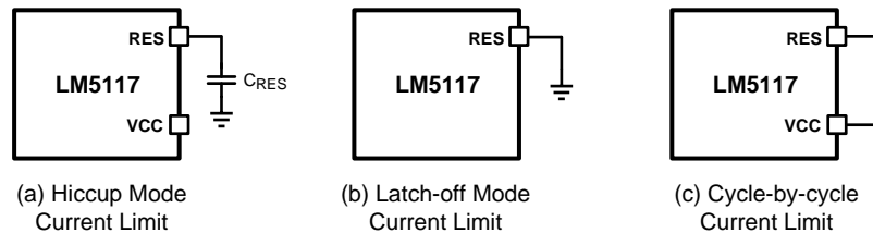
Figure 29. RES Configurations
