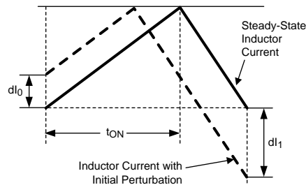
Figure 32. Effect of Initial Perturbation when dl_1/dl_0 < -1
