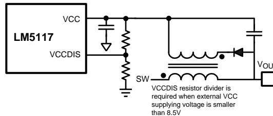
Figure 20. External VCC Supply for V_{OUT} < 6V
