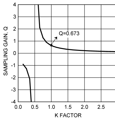
Figure 34. Sampling gain Q vs K Factor
