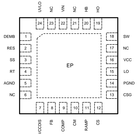
Figure 2. WQFN-24 Package (4 mm x 4 mm) (Top View)
