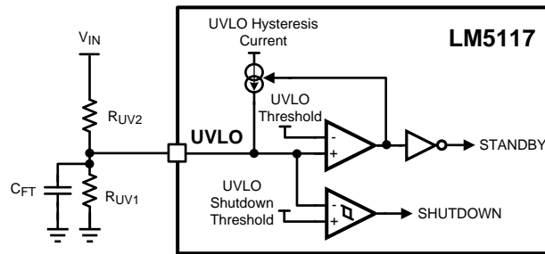
Figure 22. UVLO Configuration
