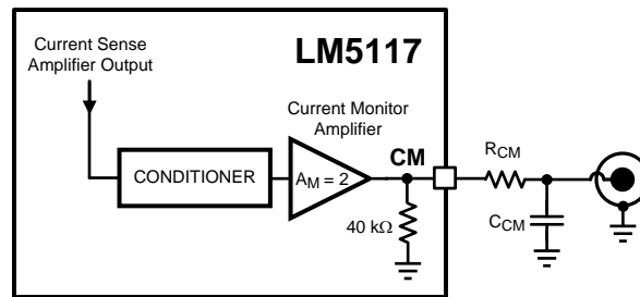
Figure 30. Current Monitor
