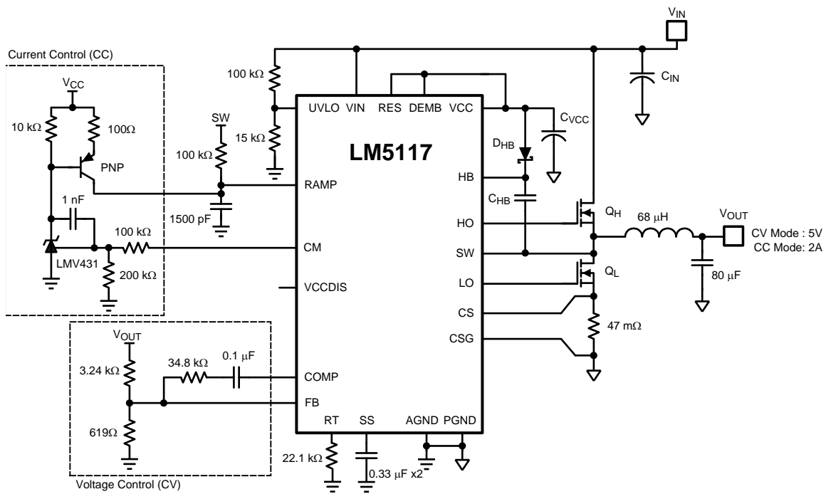
Figure 37. Constant Voltage Regulator with Accurate Current Limit
