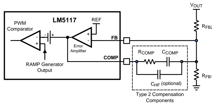
Figure 25. Feedback Configuration and PWM Comparator
