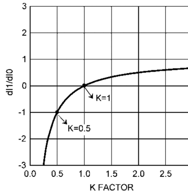
Figure 33. dl_1/dl_0 vs K Factor
