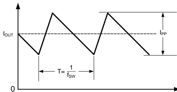
Figure 26. Inductor Current
