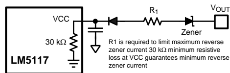
Figure 21. External VCC Supply for 14.5V < V_{OUT}
