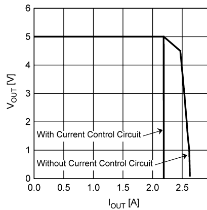
Figure 38. Current Limit Comparison
