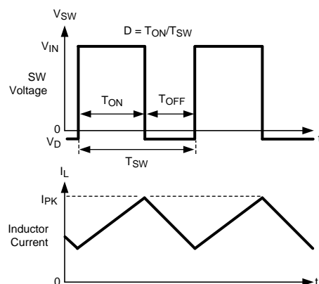
Figure 21. Typical Waveforms
