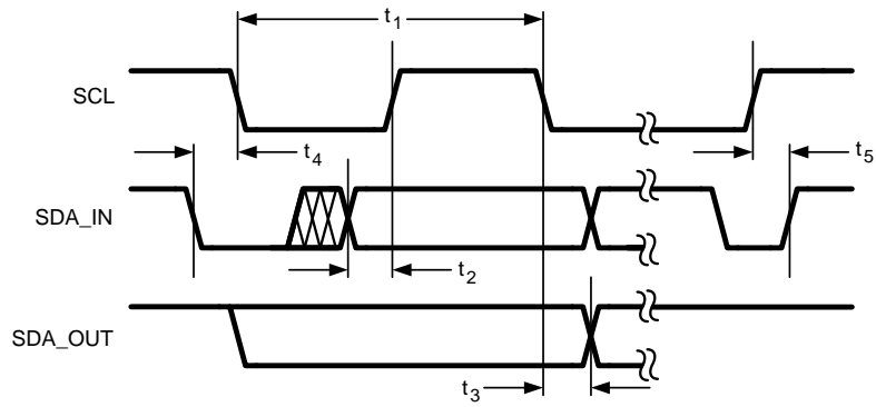
Figure 2. I 2 C-Compatible Interface Specifications
