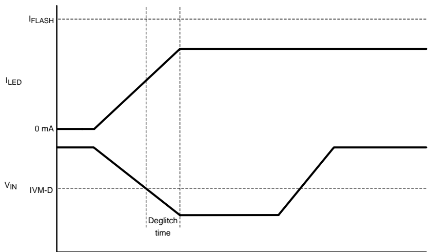
Figure 26. Stop and Hold Mode
