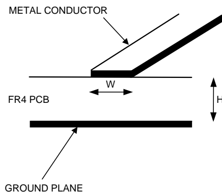
Figure 87. Microstrip Configuration
