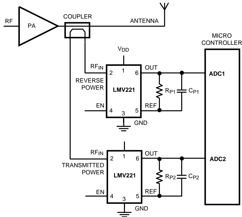
Figure 73. VSWR Application
