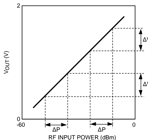
Figure 70. Linear Transfer Function
