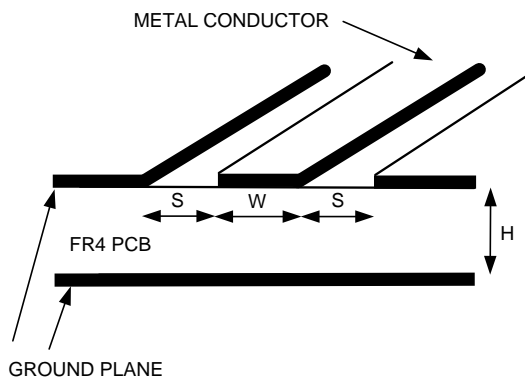
Figure 88. GCPW Configuration
