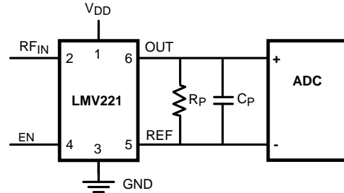
Figure 84. Differential Application
