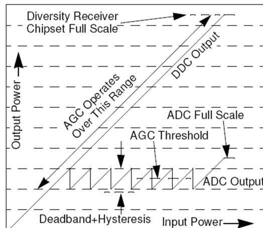
Figure 77. Output Gain Scaling vs. Input Signal
