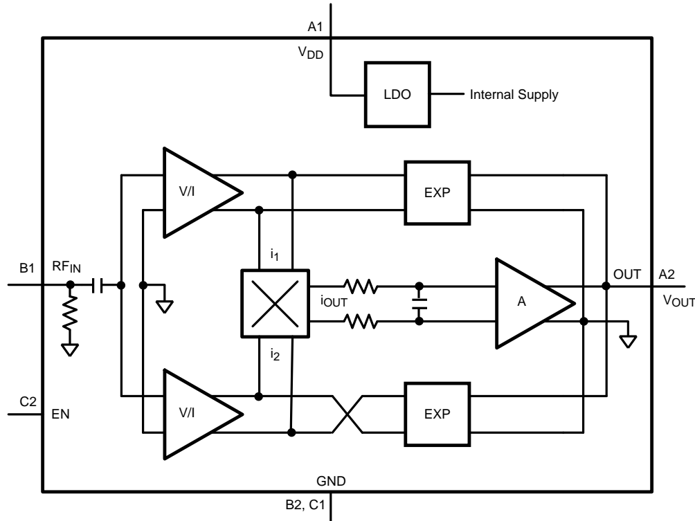
Figure 49. Block Diagram
