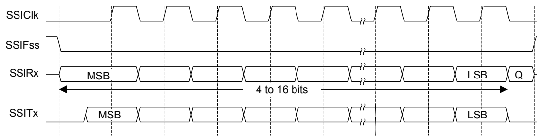
Figure 11-4. Freescale SPI Format (Single Transfer) with SPO=0 and SPH=0
