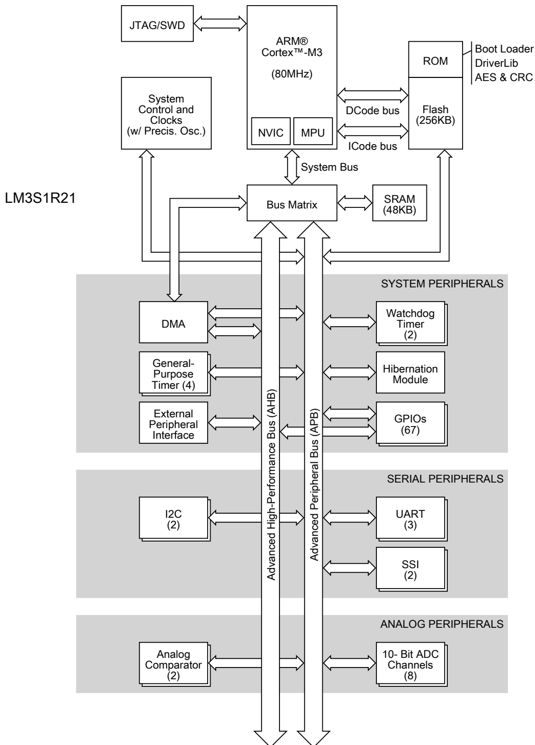
Figure 1-1. Stellaris LM3S1R21 Microcontroller High-Level Block Diagram
