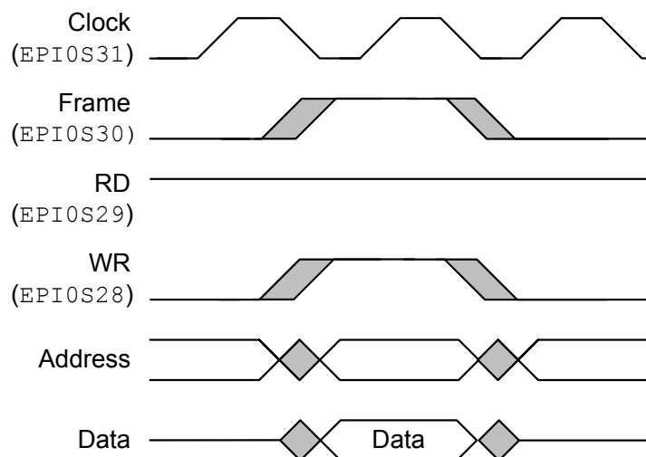
Figure 10-13. Single-Cycle Write Access, FRM50=0, FRMCNT=0, WRCYC=0
