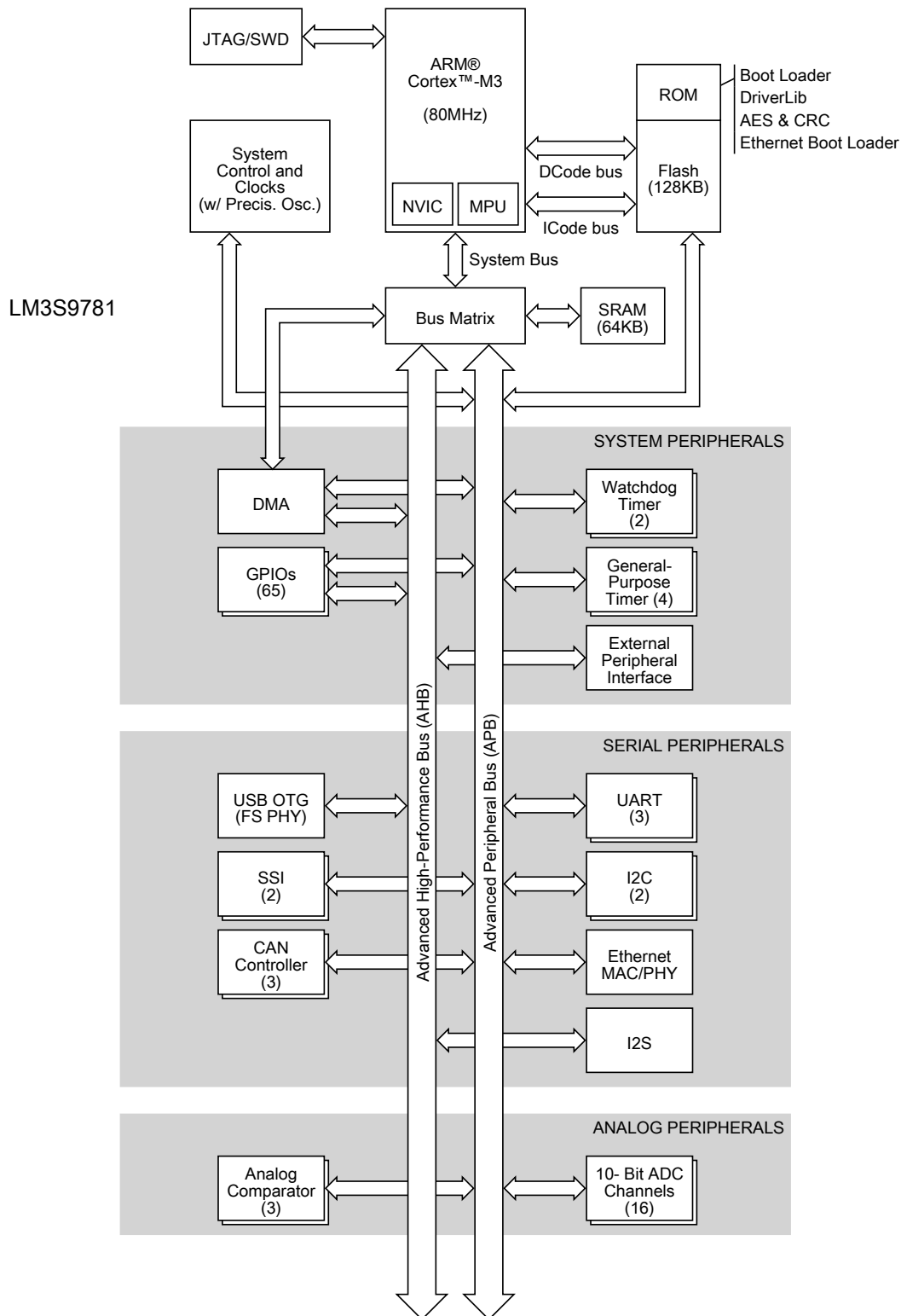
Figure 1-1. Stellaris LM3S9781 Microcontroller High-Level Block Diagram
